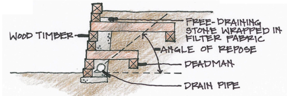
Figure 1 – Example of Deadman Use in a Retaining Wall
