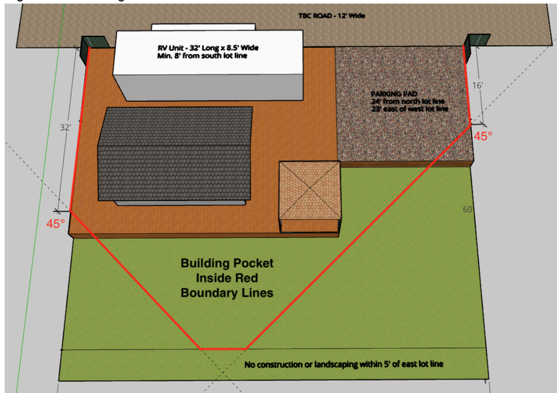
Figure 2 — Building Pocket Schematic
